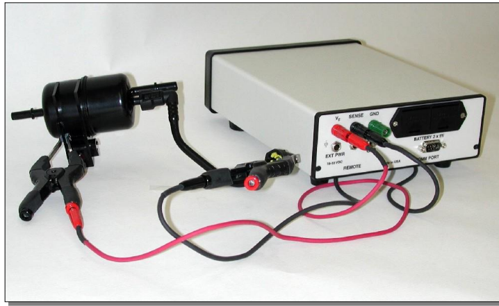
Figure 3.1-5: Connection for measuring point-to-point resistance per SAE J1645
